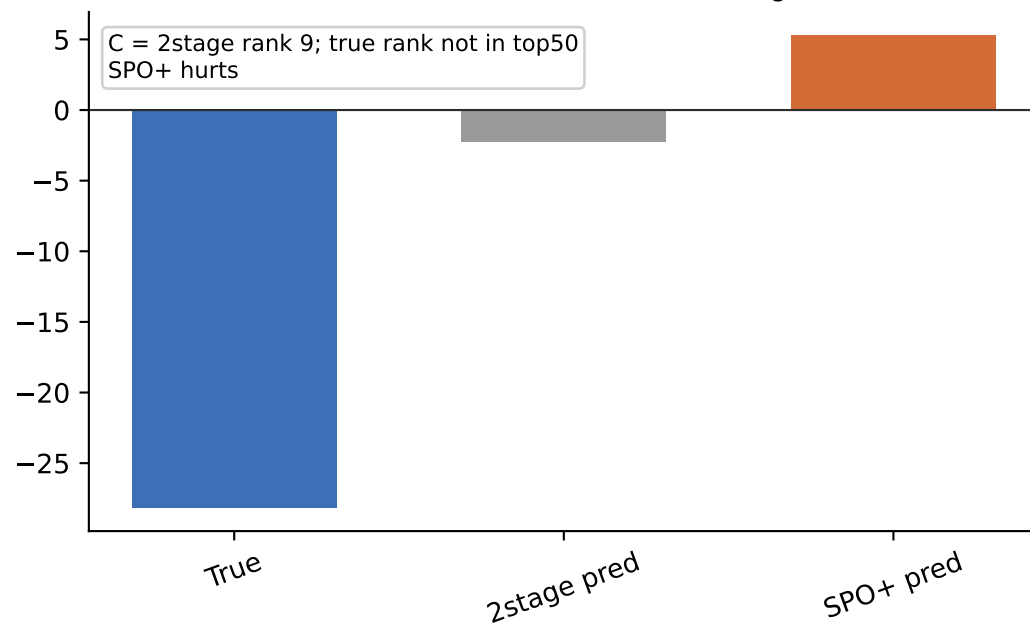
D. G-14: Harmful SPO+ reranking
